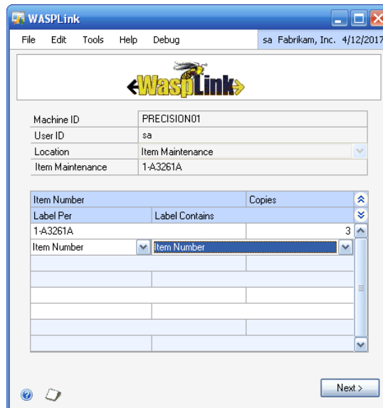
The WaspLink window preparing labels for WaspLabeler
